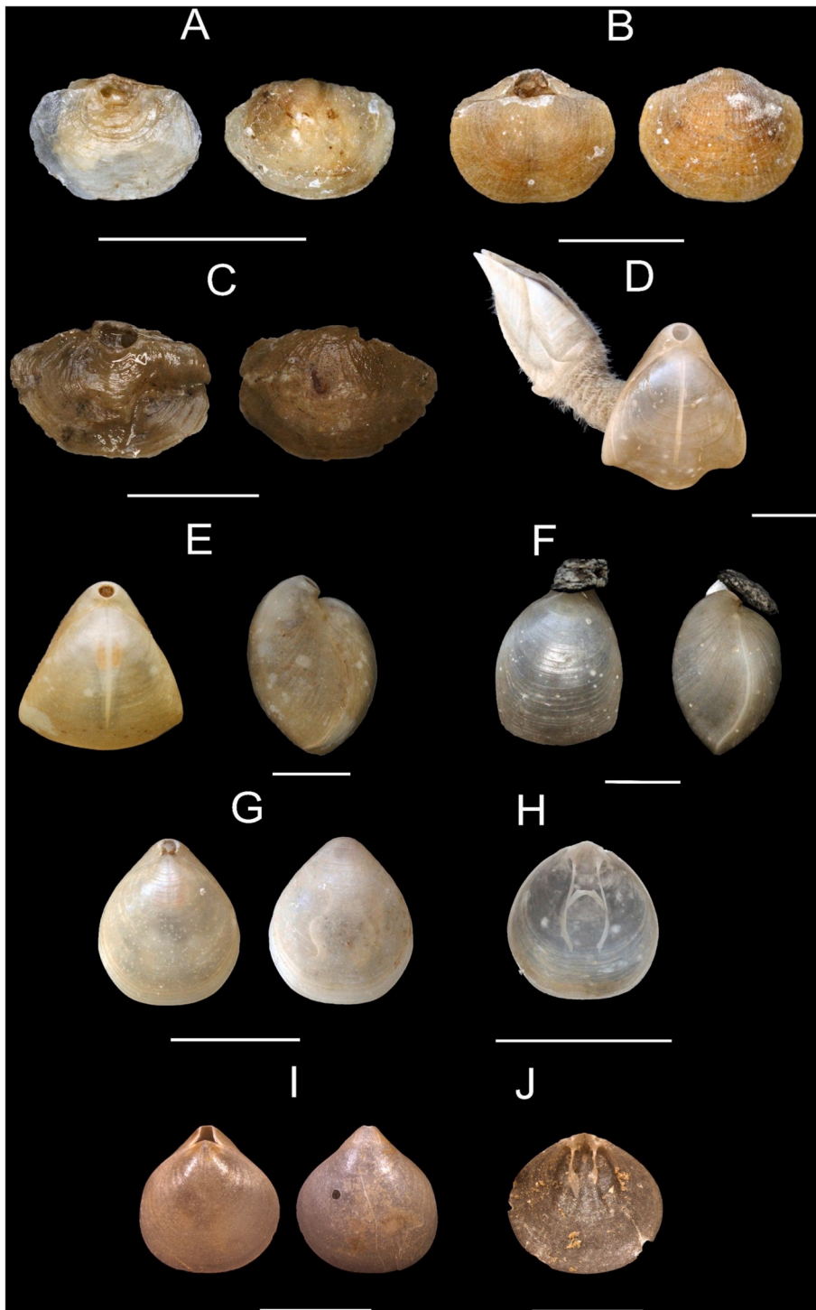
Fig. 3. Photographs of recorded brachiopod species. A, Platidia anomioides var. davidsoni , dorsal and ventral views showing small pustulas on ventral valve; B, Megerlia truncata , dorsal and ventral views; C, Megerlia truncata var. monstruosa , dorsal and ventral views; D, Dallina septigera with a barnacle of the genus Arcoscalpellum ; E, dorsal and side views of D. septigera ; F, Fallax dalliniformis , dorsal and side views; G, Macandrevia cranium dorsal and ventral views; H, interior of dorsal valve showing the brachial loop; I, Macandrevia cranium var. novangliae , dorsal and ventral views; J, brachidium of Ma. cranium var. novangliae . Scale bars A-H are 1 cm; scale bars I-J are 1 mm.
