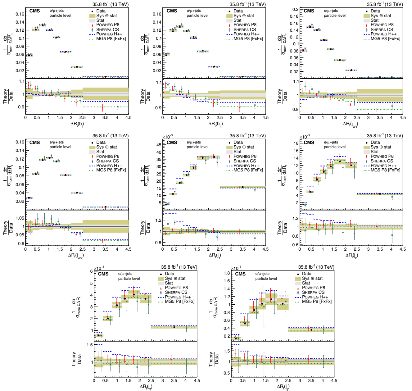
FIG. 45. Normalized differential cross section at the particle level as a function of \Delta R_j . The upper two rows show the \Delta R_j distributions for the jets in the t\bar{t} system, the lower two rows the distribution for additional jets. The data are shown as points with light (dark) bands indicating the statistical (statistical and systematic) uncertainties. The cross sections are compared to the predictions of POWHEG combined with PYTHIA8 (P8) or HERWIG++ (H++) and the multiparton simulations MG5_AMC@NLO (MG5)+PYTHIA8 FxFx and SHERPA. The ratios of the predictions to the measured cross sections are shown at the bottom of each panel.
