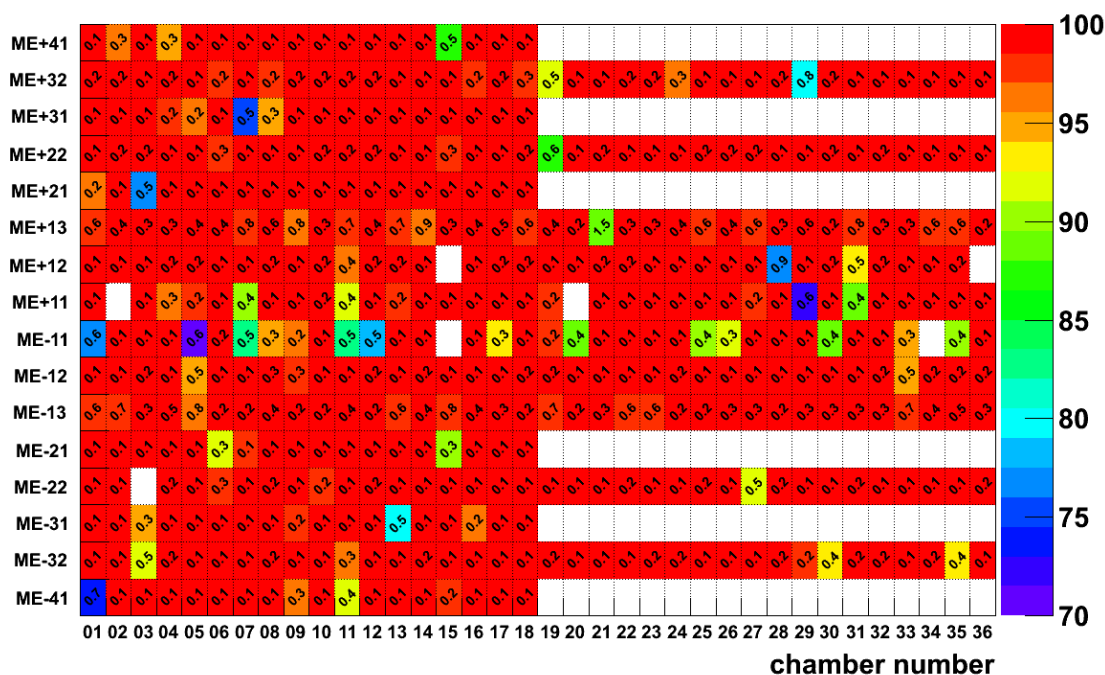
CSC Rechit efficiency (in %) CMS 2010 \sqrt{s} = 7 TeV
