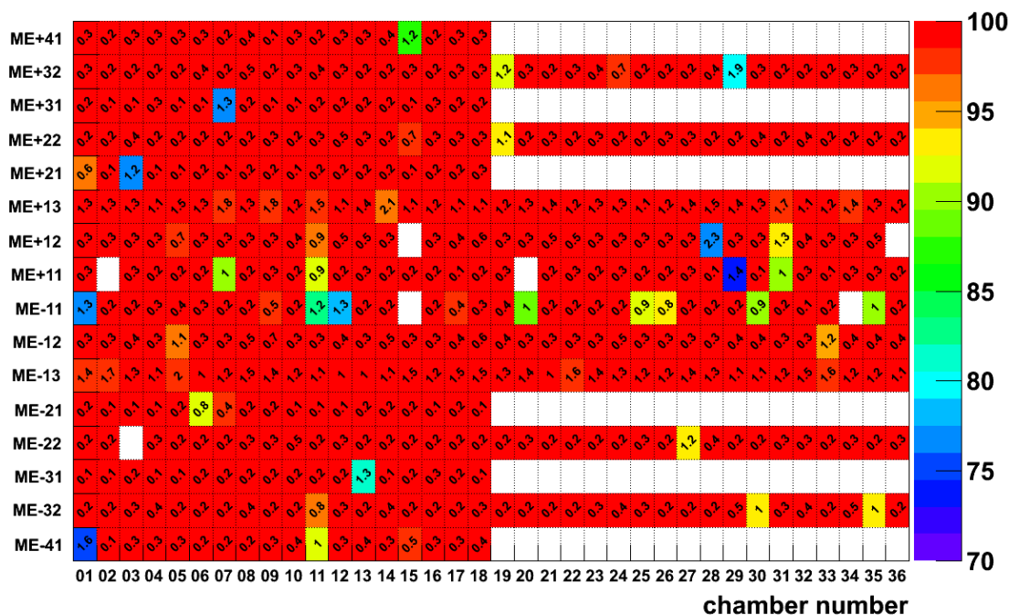
CSC Segment efficiency (in %) CMS 2010 \sqrt{s} = 7 TeV
