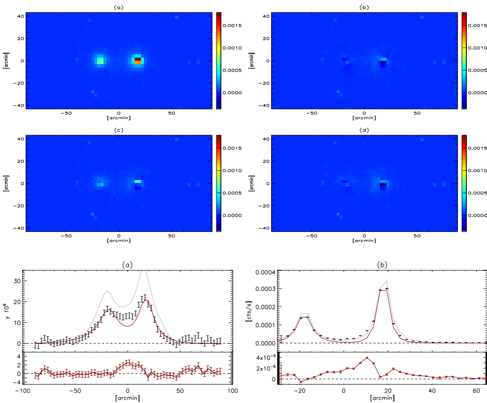
Fig. 5. X-ray data and residuals of the best-fit cluster model for the A399 and A401 pair of clusters. a) ROSAT map; b) residuals for the GNF2 model; c) residuals for the GNF1 model; and d) residuals for the \beta model.
