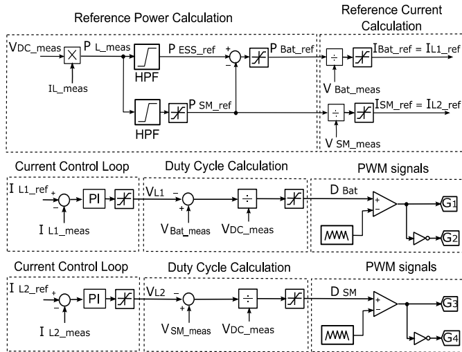
Fig. 3. Control of the Parallel Connection (PC) in order to provide or absorb transient power during load variations in order to improve the recovery of the DC link due to load variations.
