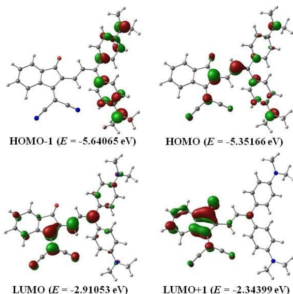
Fig. 8 Frontier orbitals for compound 4f .
