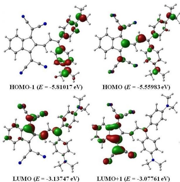
Fig. 9 Frontier orbitals for compound 5f .
