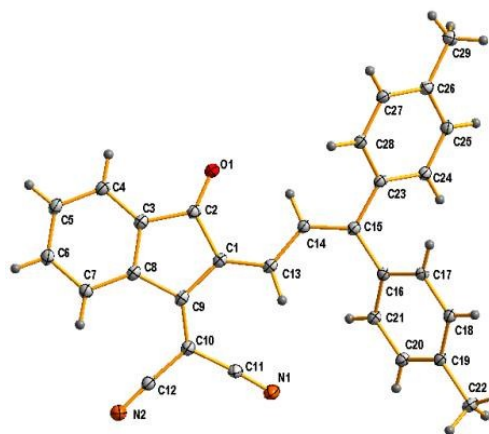
Fig. 3 ORTEP-type view of the structure of 4d showing the crystallographic labelling scheme. Thermal ellipsoids are drawn at 30% probability level. Selected bond distances (Å): C(2)-O(1) = 1.221(2), C(9)-C(10) = 1.369(2), C(10)-C(11) = 1.444(2), C(10)-C(12) = 1.437(2), C(11)-N(1) = 1.154(2), C(12)-N(2) = 1.417(2), C(1)-C(13) = 1.376(2), C(13)-C(14) = 1.417(2), C(14)-C(15) = 1.373(2). Selected bond angles ( ^\circ ): C(2)-C(1)-C(9) = 106.9(1), C(2)-C(1)-C(13) = 124.6(2), C(9)-C(1)-C(13) = 128.3(2), C(1)-C(13)-C(14) = 123.6(1), C(13)-C(14)-C(15) = 127.4(1), C(14)-C(15)-C(16) = 125.8(1), C(14)-C(15)-C(23) = 116.8(1), C(10)-C(11)-N(1) = 176.2(2), C(10)-C(12)-N(2) = 177.1(2).
