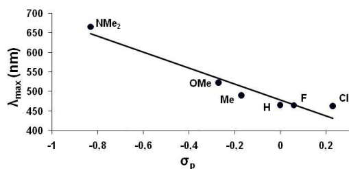
Fig. 6 Plot of \lambda_{\max} vs Hammett coefficients for compounds 4a-f .
