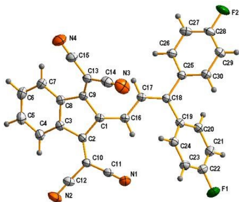
Fig. 4 ORTEP-type view of the structure of 5b showing the crystallographic labelling scheme. Thermal ellipsoids are drawn at 30% probability level. Selected bond distances (Å): C(2)-C(10) = 1.358(2), C(10)-C(11) = 1.431(2), C(10)-C(12) = 1.428(2), C(11)-N(1) = 1.148(2), C(12)-N(2) = 1.137(2), C(9)-C(13) = 1.360(2), C(13)-C(14) = 1.429(2), C(13)-C(15) = 1.431(2), C(14)-N(3) = 1.143(2), C(15)-N(4) = 1.136(2), C(1)-C(16) = 1.359(2), C(16)-C(17) = 1.430(2), C(17)-C(18) = 1.360(2). Selected bond angles (°): C(2)-C(1)-C(9) = 105.3(1), C(9)-C(1)-C(16) = 128.1(1), C(2)-C(1)-C(16) = 124.5(1), C(1)-C(16)-C(17) = 126.5(1), C(16)-C(17)-C(18) = 124.9(1), C(17)-C(18)-C(19) = 121.4(1), C(17)-C(18)-C(25) = 120.3(1), C(10)-C(11)-N(1) = 176.9(1), C(10)-C(12)-N(2) = 176.8(2), C(13)-C(14)-N(3) = 175.7(2), C(13)-C(15)-N(4) = 178.6(2).
