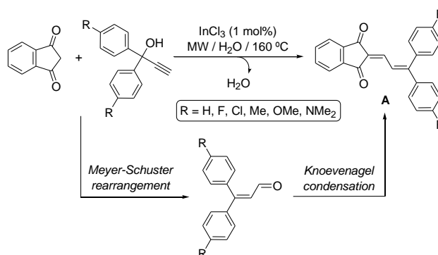
Scheme 1 Synthesis of butadiene dyes from indan-1,3-dione and terminal alkynols.
