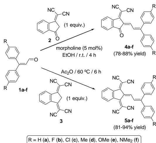
Scheme 2 Synthesis of butadiene dyes 4a-f and 5a-f .
