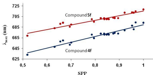
Fig. 7 Plot of \lambda_{\max} vs SPP values for compounds 4-5f .
