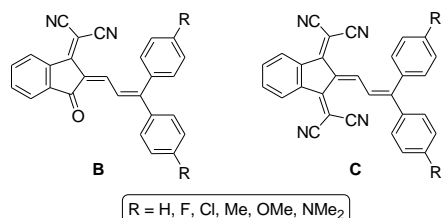
Fig. 2 Structure of the butadiene dyes synthesized in this work.
