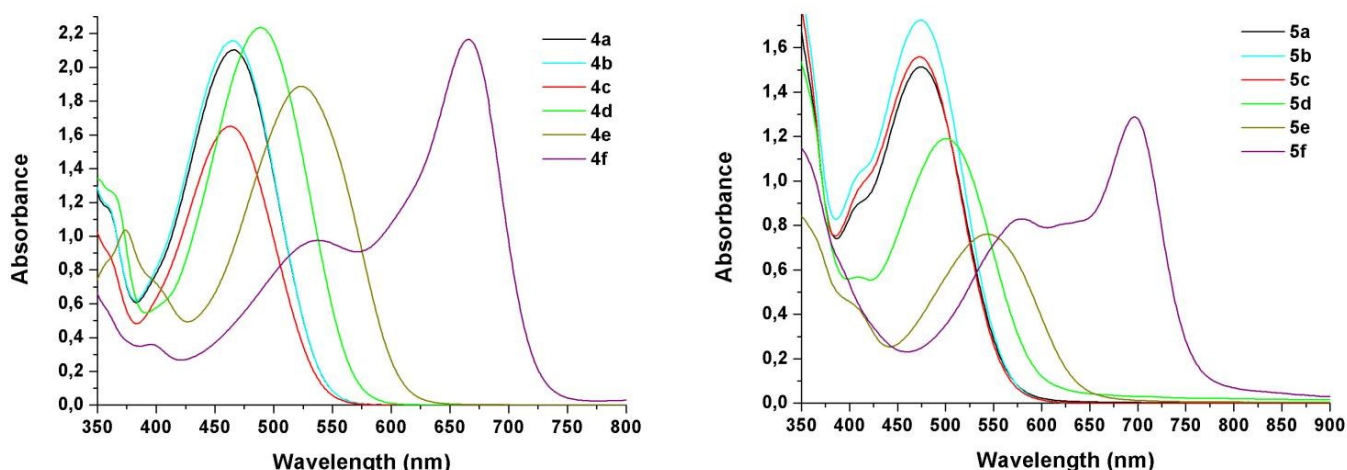
Fig. 5 UV-Vis spectra of the butadiene dyes 4a-f (left) and 5a-f (right) recorded in 6 \times 10^{-5} M dichloromethane solution.
