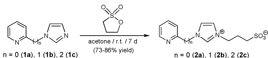
Scheme 1. Synthesis of the zwitterionic imidazolium salts 2a-c .
