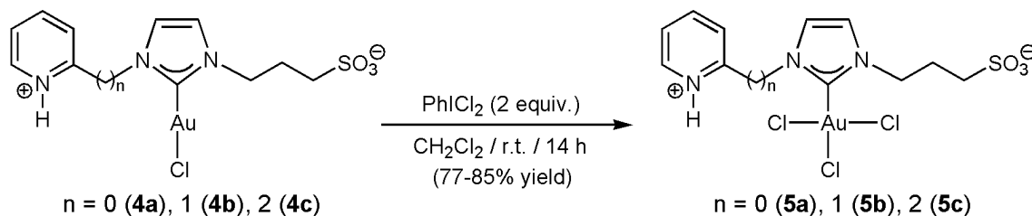
Scheme 3. Synthesis of the NHC-Au(III) complexes 5a-c .
