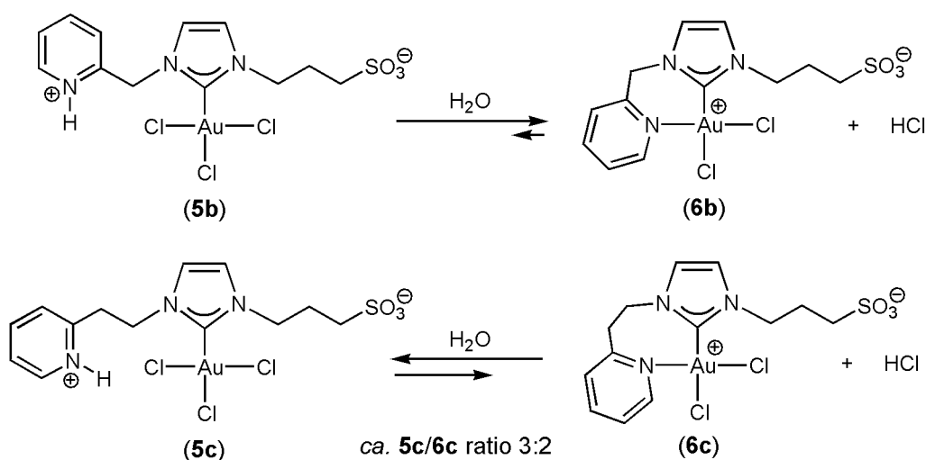
Scheme 4. The behavior of the NHC-Au(III) complexes 5b-c in water.
