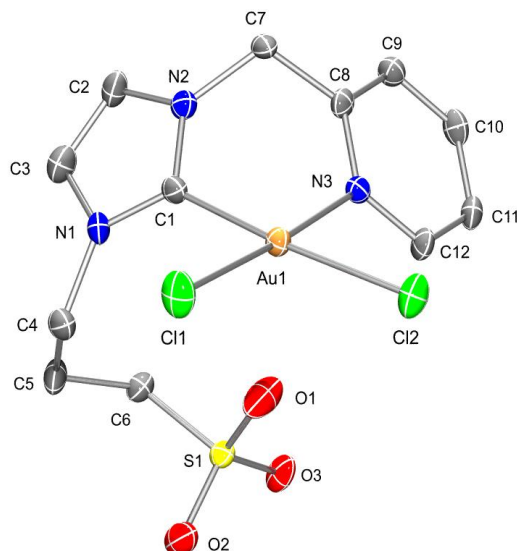
Figure 5. ORTEP-type view of the structure of the NHC-Au(III) complex 6b showing the crystallographic labelling scheme. Thermal ellipsoids are drawn at 50% probability level. Hydrogen atoms have been omitted for clarity. Selected bond distances (Å) and angles (deg): Au(1)-C(1) = 2.006(6); Au(1)-Cl(1) = 2.2767(13); Au(1)-Cl(2) = 2.23194(14); Au(1)-N(3) = 2.053(4); C(1)-N(1) = 1.347(8); C(1)-N(2) = 1.325(7); C(2)-N(2) = 1.381(7); C(2)-C(3) = 1.351(10); C(3)-N(1) = 1.390(8); C(1)-Au(1)-Cl(1) = 92.42(17); C(1)-Au(1)-Cl(2) = 175.22(17); C(1)-Au(1)-N(3) = 85.7(2); Cl(1)-Au(1)-Cl(2) = 91.83(5); Cl(1)-Au(1)-N(3) = 176.37(13); Cl(2)-Au(1)-N(3) = 89.93(13); N(1)-C(1)-N(2) = 107.8(5); C(1)-N(2)-C(2) = 110.1(5); N(2)-C(2)-C(3) = 106.4(5); C(2)-C(3)-N(1) = 107.5(6); C(3)-N(1)-C(1) = 108.2(5).
