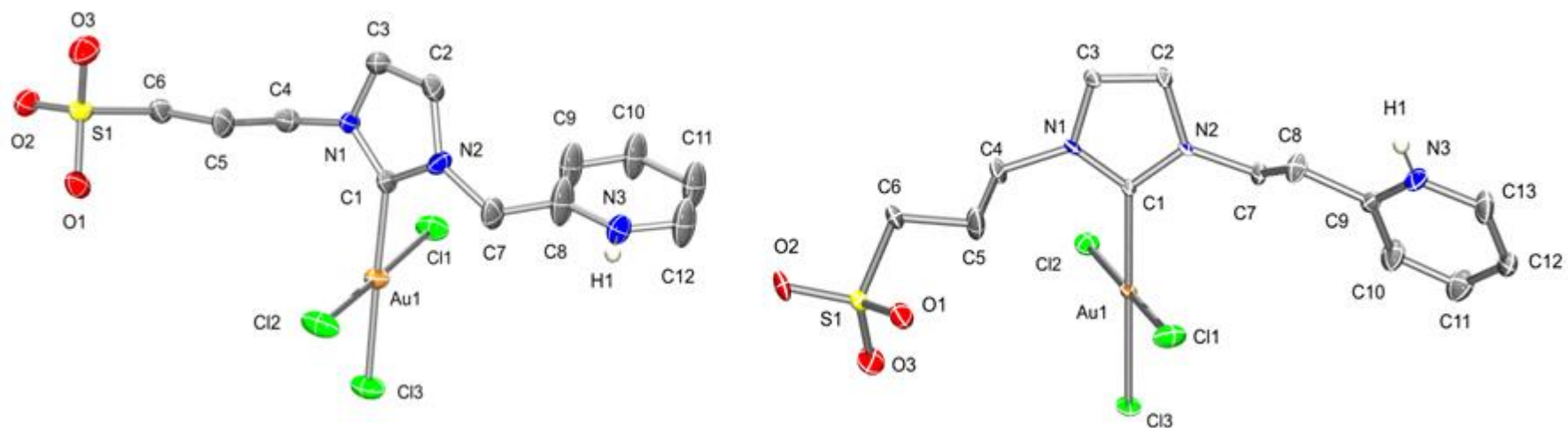
Figure 4. ORTEP-type views of the structures of the NHC-Au(III) complexes 5b (left) and 5c (right) showing the crystallographic labelling scheme. Thermal ellipsoids are drawn at 50% ( 5b ) and 30% ( 5c ) probability level. Hydrogen atoms, except those on the N(3) atoms, have been omitted for clarity.
