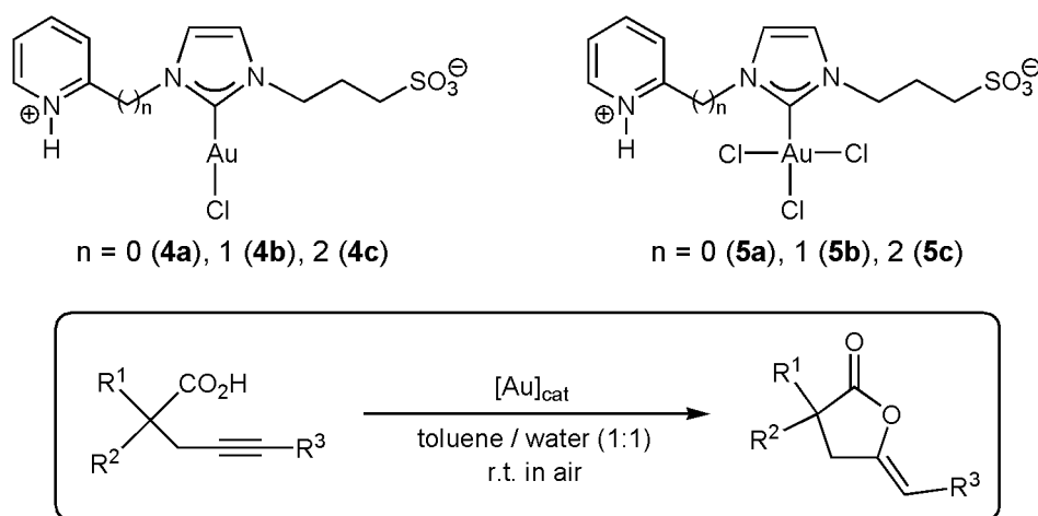
Figure 2. Structure of the gold-NHC complexes described in this work and the cycloisomerization reaction of \gamma -alkynoic acids.
