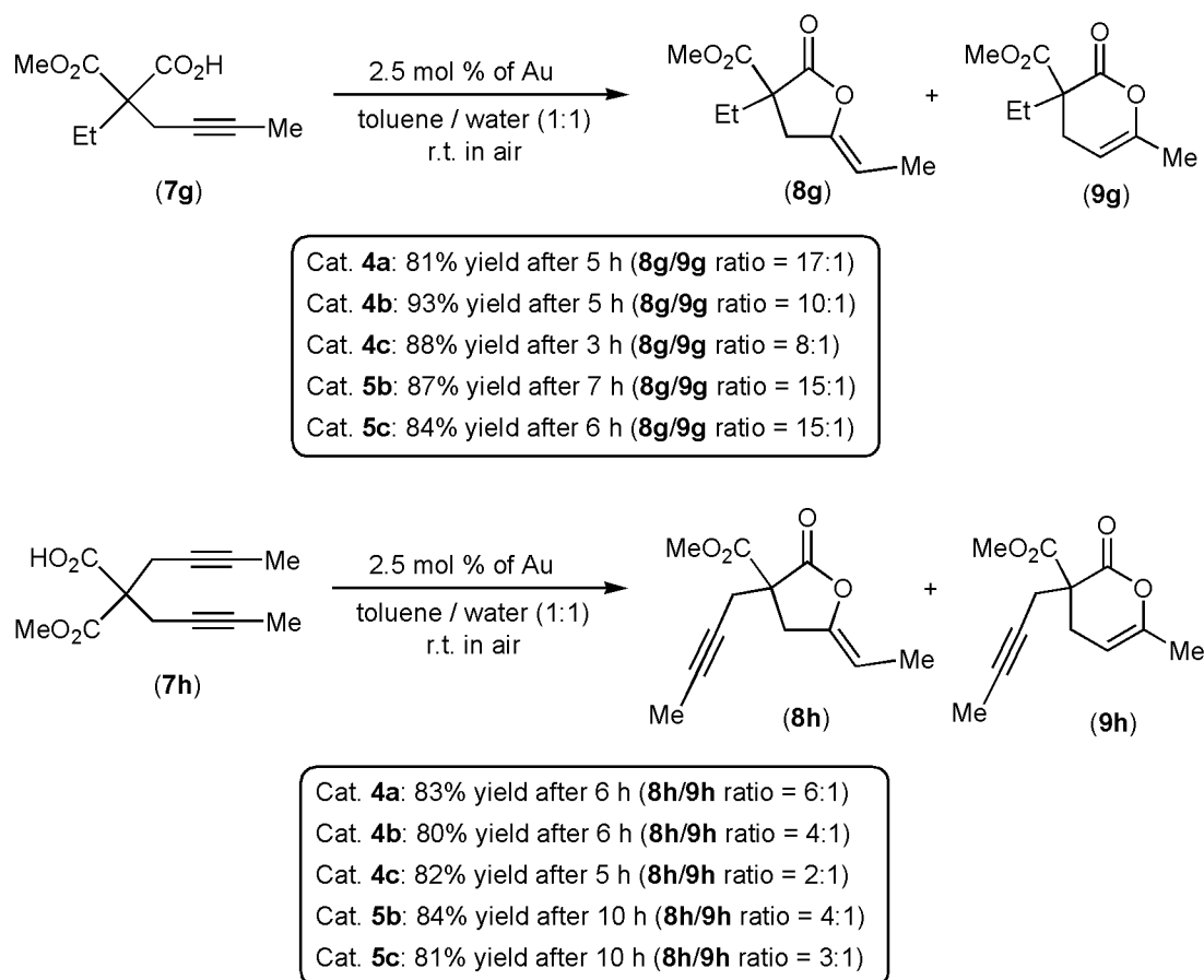
Scheme 5. Catalytic cycloisomerization of the alkynoic acids 7g-h by complexes 4a-c and 5b-c .
