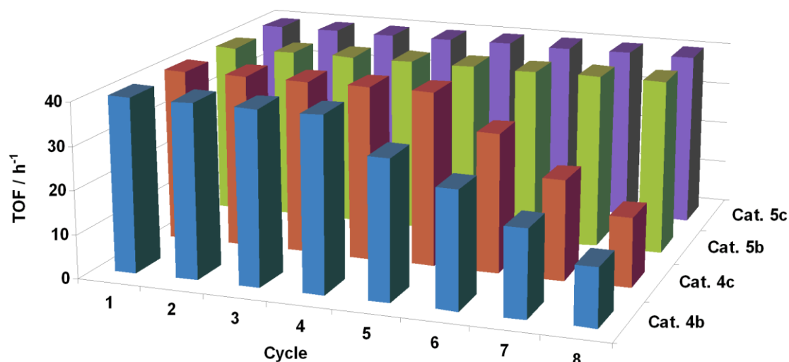
Figure 6. Evolution of the turnover frequency (TOF) of catalysts 4-5b-c during recycling.
