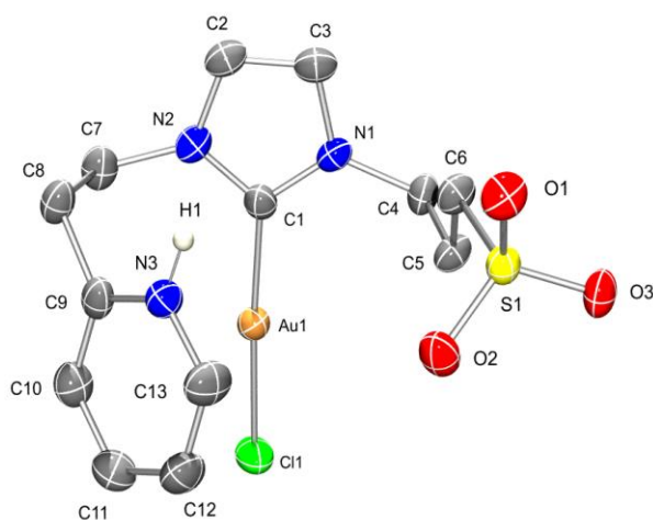
Figure 3. ORTEP-type view of the structure of the NHC-Au(I) complex 4c showing the crystallographic labelling scheme. Thermal ellipsoids are drawn at 50% probability level. Hydrogen atoms, except that on N(3), have been omitted for clarity. Selected bond distances (Å) and angles (deg): Au(1)-C(1) = 1.988(5); Au(1)-Cl(1) = 2.2856(14); C(1)-N(1) = 1.339(7); C(1)-N(2) = 1.352(6); C(2)-N(2) = 1.387(8); C(2)-C(3) = 1.346(8); C(3)-N(1) = 1.389(7); C(1)-Au(1)-Cl(1) = 176.37(15); N(1)-C(1)-N(2) = 105.3(4); C(1)-N(2)-C(2) = 110.4(4); N(2)-C(2)-C(3) = 106.8(5); C(2)-C(3)-N(1) = 106.5(5); C(3)-N(1)-C(1) = 111.0(4).
